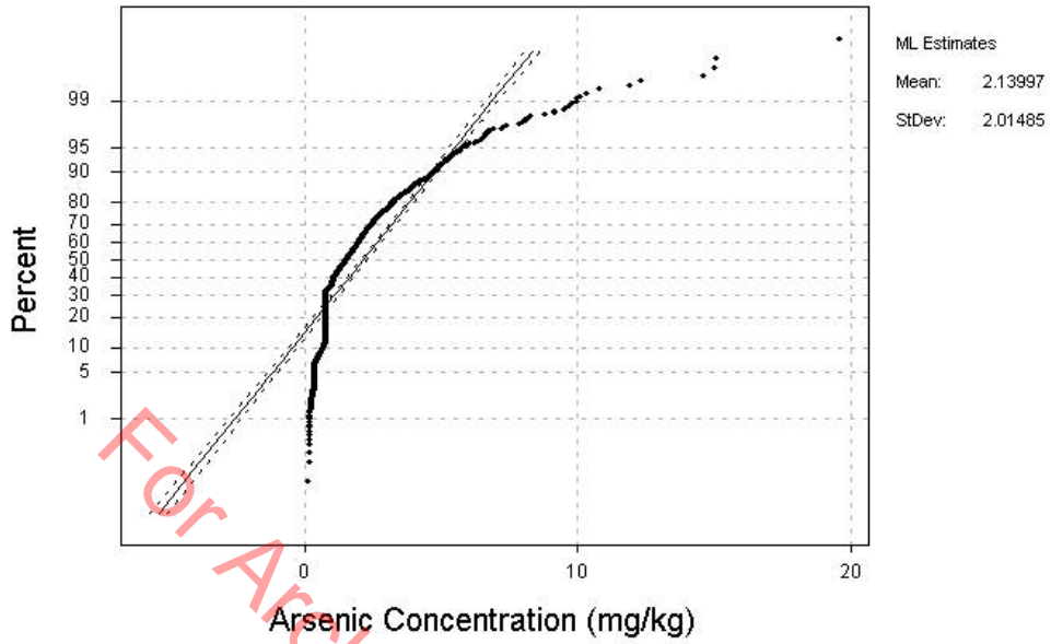
Normal Probability Plot for Arsenic Data
