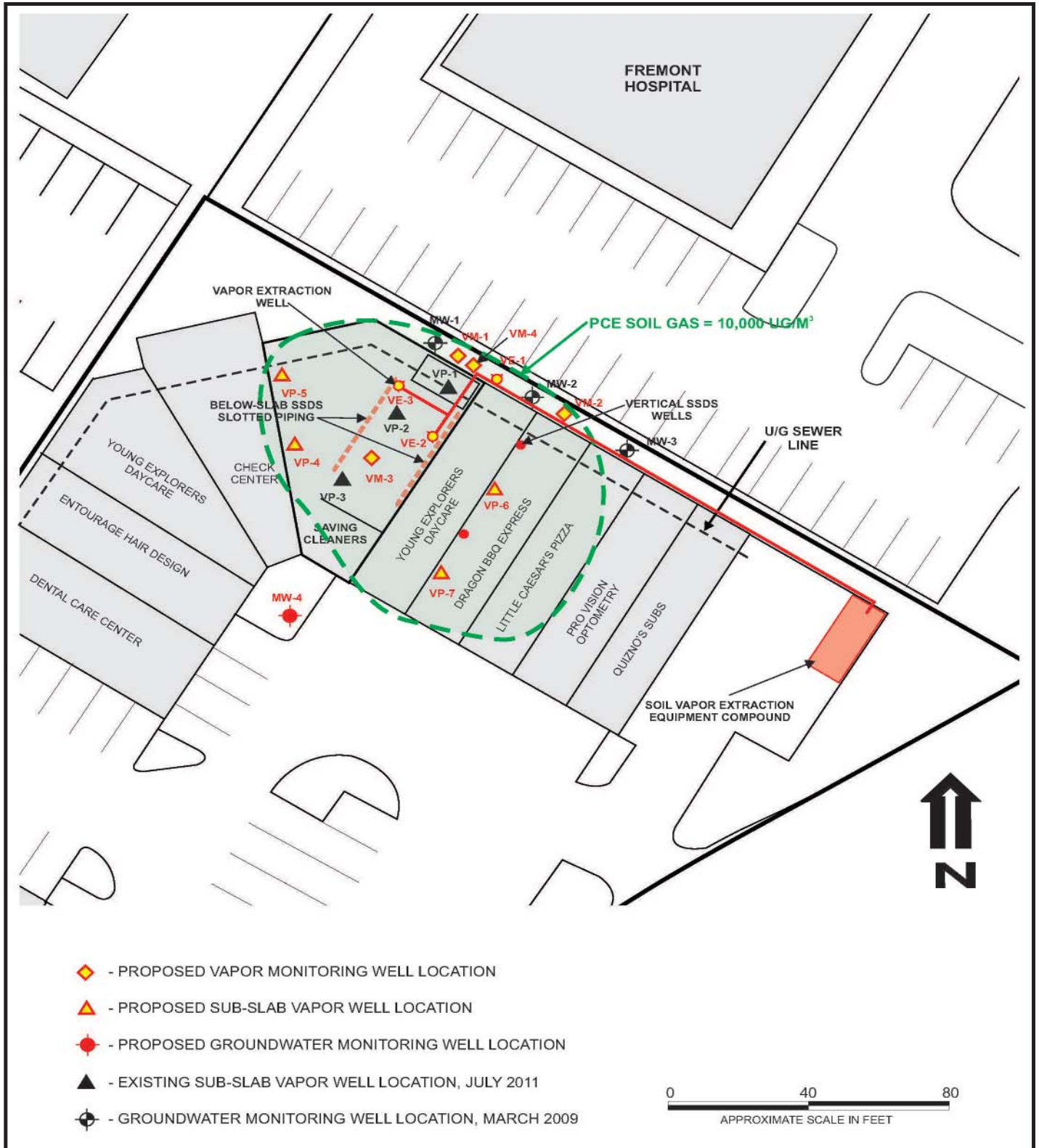
Figure 1 Saving Cleaners Site Conceptual Remediation System Implementation Layout
